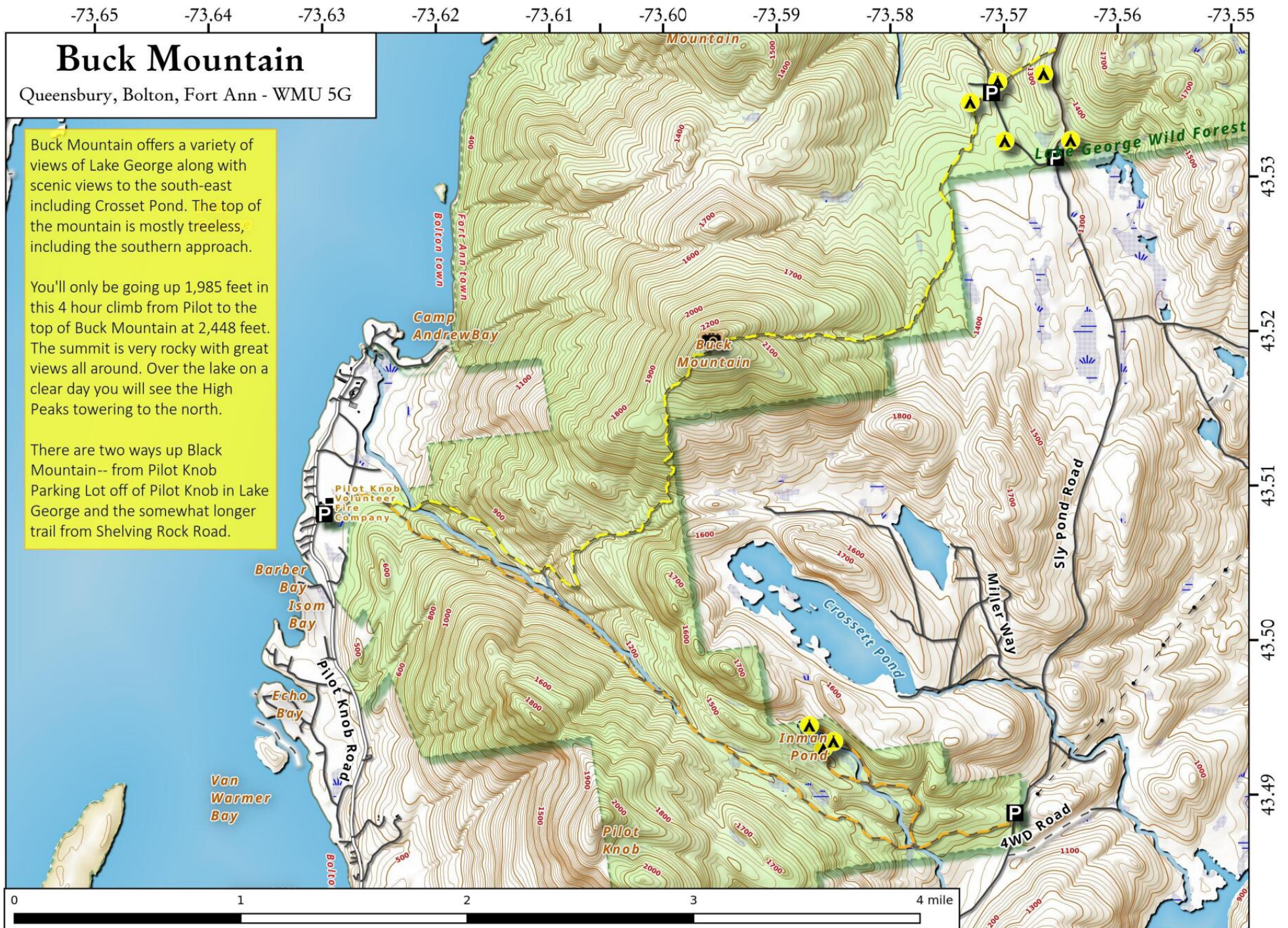
Buck Mountain Map, December 8, 2017 by AndyArthur.org in QGIS 2.18.11 and Python. Street Map is Copyright © OpenStreetMap contributors, CC BY-SA. NYSDEC Data: DEM, Borders, ADK Wetlands, Trails, Assets. True North. 1 inch = 0.5 miles. Projection: NAD83 / UTM zone 18N. Coordinates: 0.01° latitude-longitude (WGS84). Contours are 20 feet.
