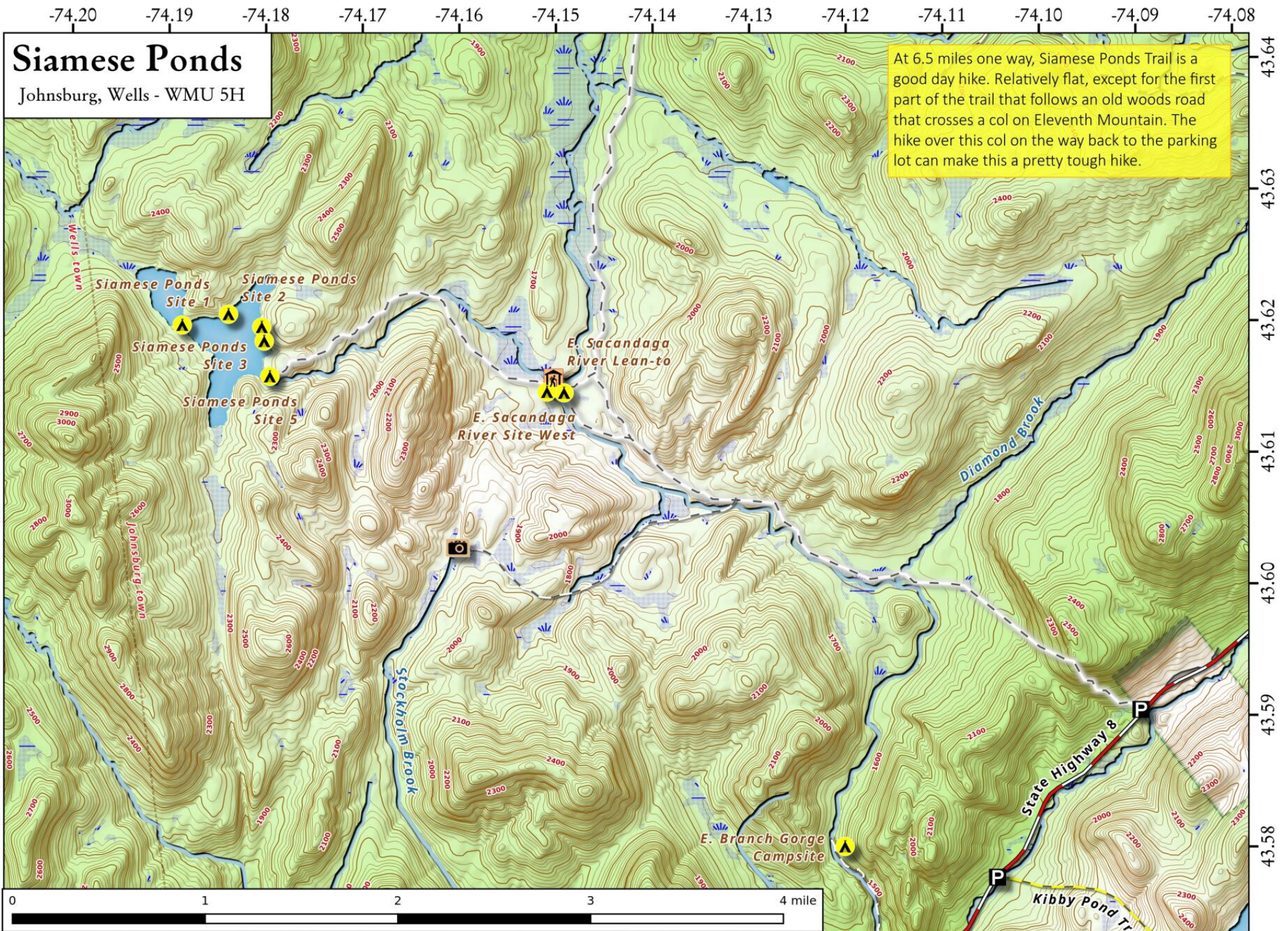
Siamese Ponds Map, March 25, 2017 by AndyArthur.org in QGIS 2.18.3 and Python. Street Map is Copyright © OpenStreetMap contributors, CC BY-SA. NYSDEC Data: DEM, Borders, ADK Wetlands, Trails, Assets. True North. 1 inch = 0.6 miles. Projection: NAD83 / UTM zone 18N. Coordinates: 0.01° latitude-longitude (WGS84). Contours are 20 feet.
