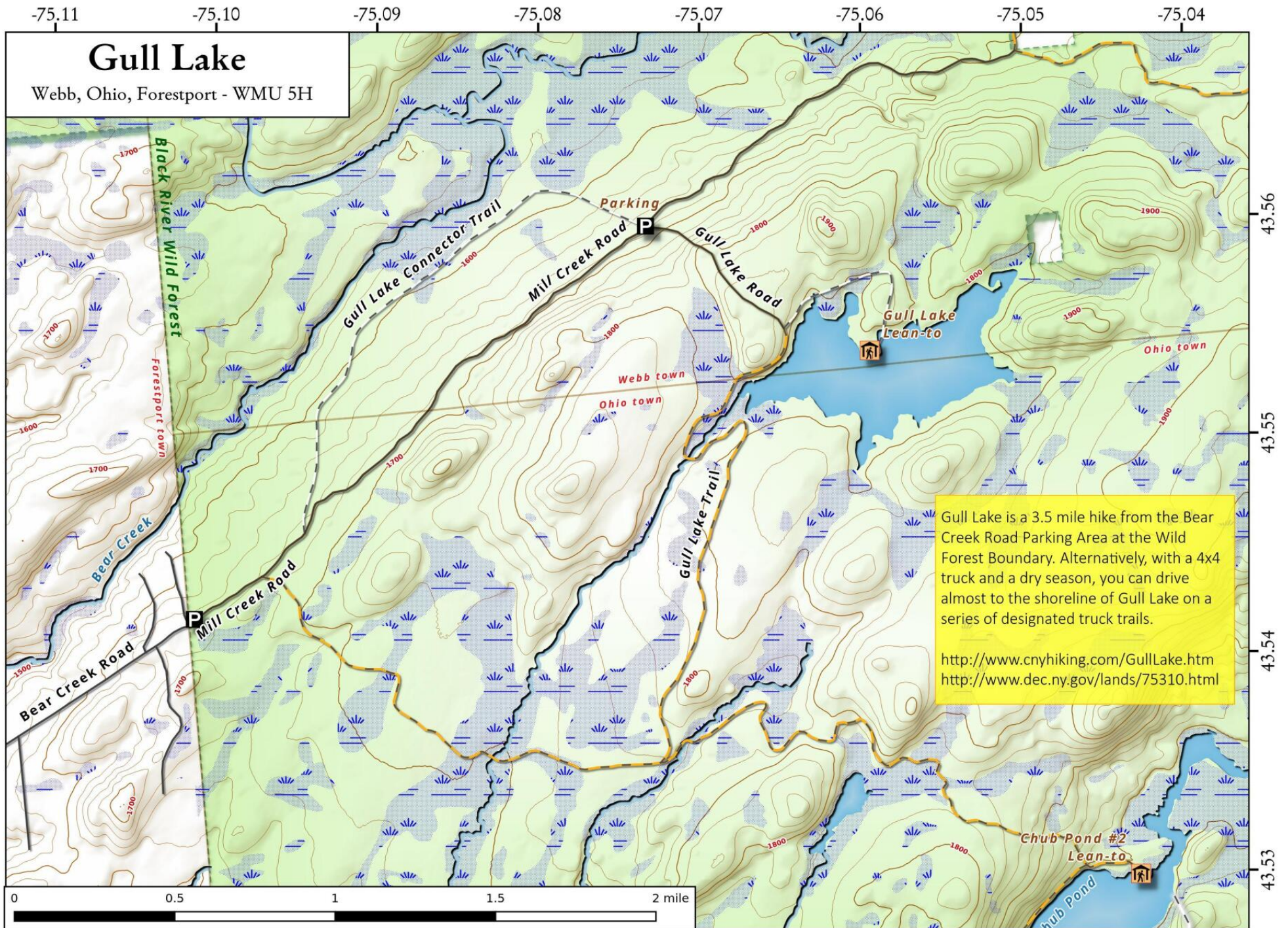
Gull Lake Map, July 5, 2017 by AndyArthur.org in QGIS 2.18.9 and Python. Street Map is Copyright © OpenStreetMap contributors, CC BY-SA. NYSDEC Data: DEM, Borders, ADK Wetlands, Trails, Assets. True North. 1 inch = 0.4 miles. Projection: NAD83 / UTM zone 18N. Coordinates: 0.01° latitude-longitude (WGS84). Contours are 20 feet.
