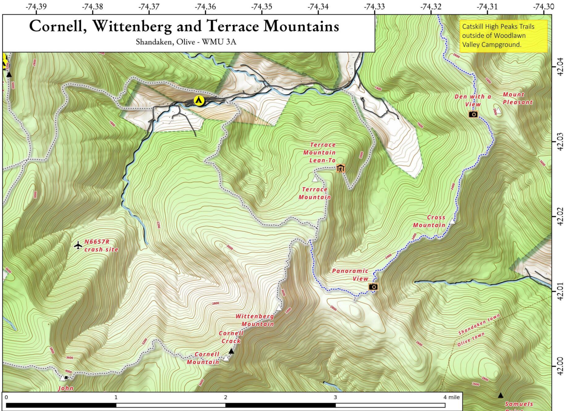
Cornell, Wittenberg and Terrace Mountains Map, January 2, 2017 by AndyArthur.org in QGIS 2.18.2 and Python. Street Map is Copyright © OpenStreetMap contributors, CC BY-SA. NYSDEC Data: DEM, Borders, ADK Wetlands, Trails, Assets. True North. 1 inch = 0.5 miles. Projection: NAD83 / UTM zone 18N. Coordinates: 0.01° latitude-longitude (WGS84). Contours are 40 feet.
