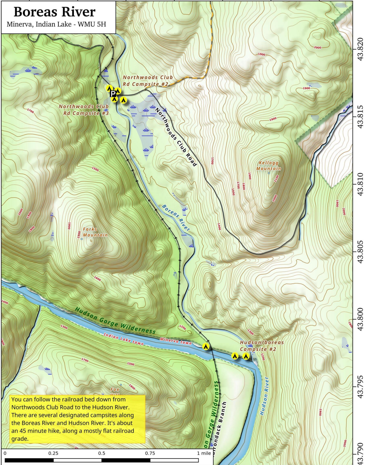
Boreas River Map, May 23, 2017 by AndyArthur.org in QGIS 2.18.7 and Python. Street Map is Copyright © OpenStreetMap contributors, CC BY-SA. NYSDEC Data: DEM, Borders, ADK Wetlands, Trails, Assets. True North. 1 inch = 0.2 miles. Projection: NAD83 / UTM zone 18N. Coordinates: 0.005° latitude-longitude (WGS84). Contours are 20 feet.
