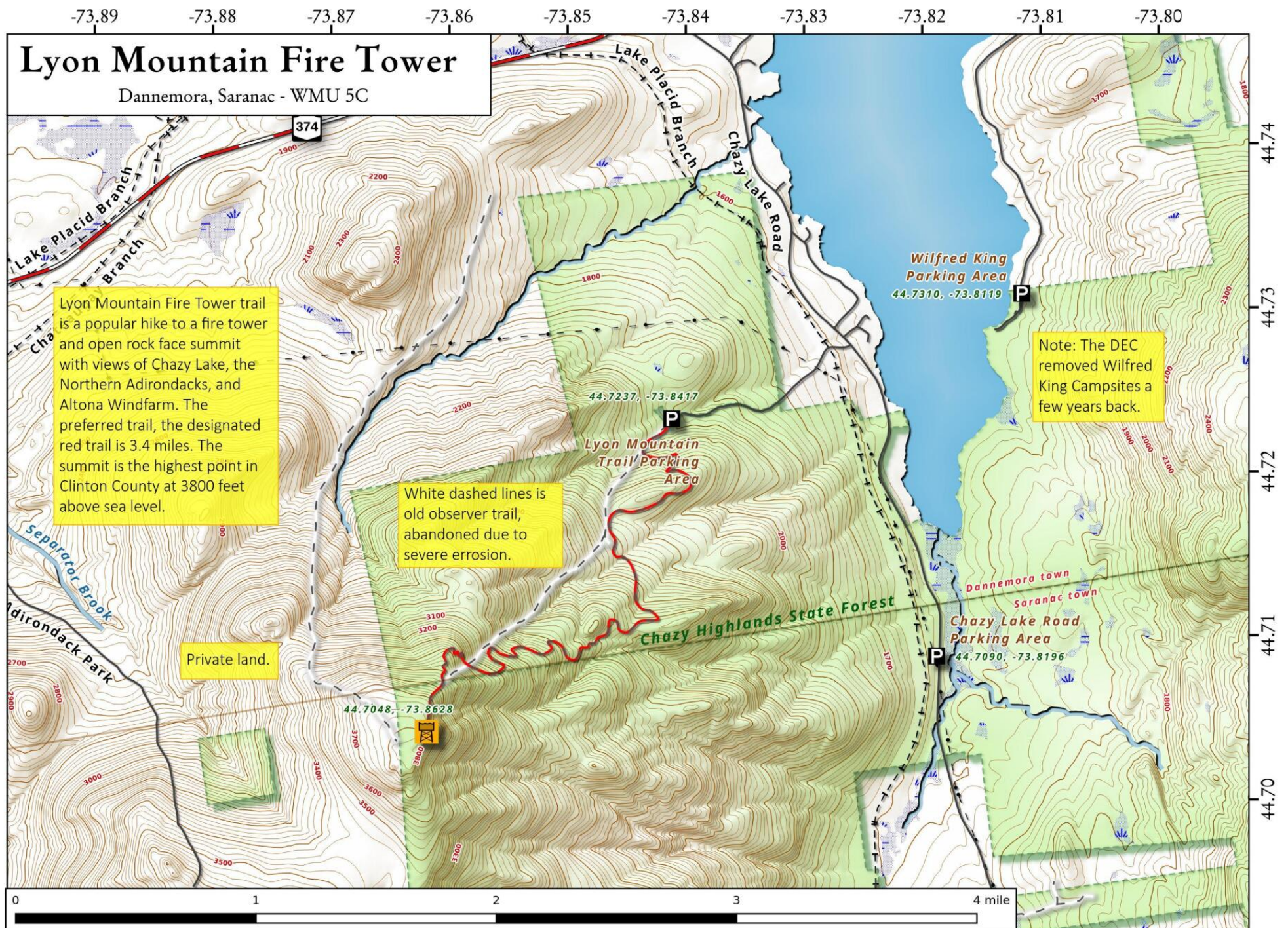
Lyon Mountain Fire Tower Map, September 10, 2017 by AndyArthur.org in QGIS 2.18.11 and Python. Street Map is Copyright © OpenStreetMap contributors, CC BY-SA. NYSDEC Data: DEM, Borders, ADK Wetlands, Trails, Assets. True North. 1 inch = 0.5 miles. Projection: NAD83 / UTM zone 18N. Coordinates: 0.01° latitude-longitude (WGS84). Contours are 20 feet.
